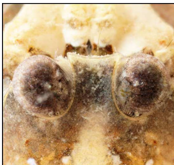
Philocheras sculptus
