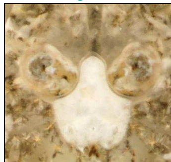
Philocheras trispinosus
