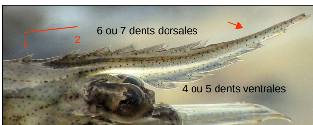
Palaemon serratus
