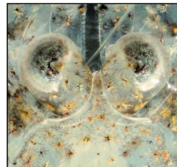
Crangon crangon
