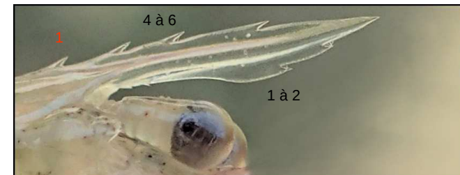
Palaemon varians
